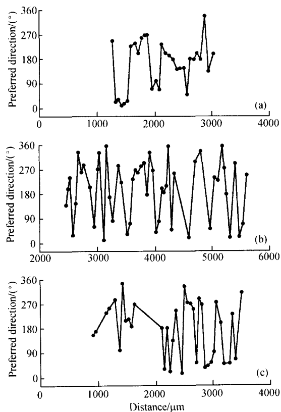
Fig. 3. Plots illustrating the change in cortical cells' preferred direction with the distance along microelectrode penetrations. (a) A penetration vertically through area 17 of a cat; (b) a penetration horizontally through V1 of a monkey; (c) a penetration vertically through V1 of a monkey. Note that in general, preferred directions of successively recorded cells were similar, but often interspersed with many reversals of approximately 180 degrees in between. This phenomenon was more significant in monkeys than in cats.
