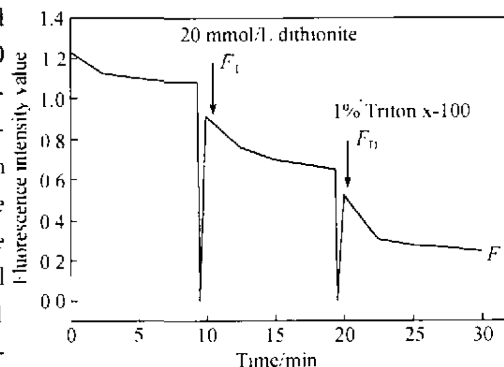
Fig. 1 Principle of assay for phospholipid flippase in plasma membrane.
