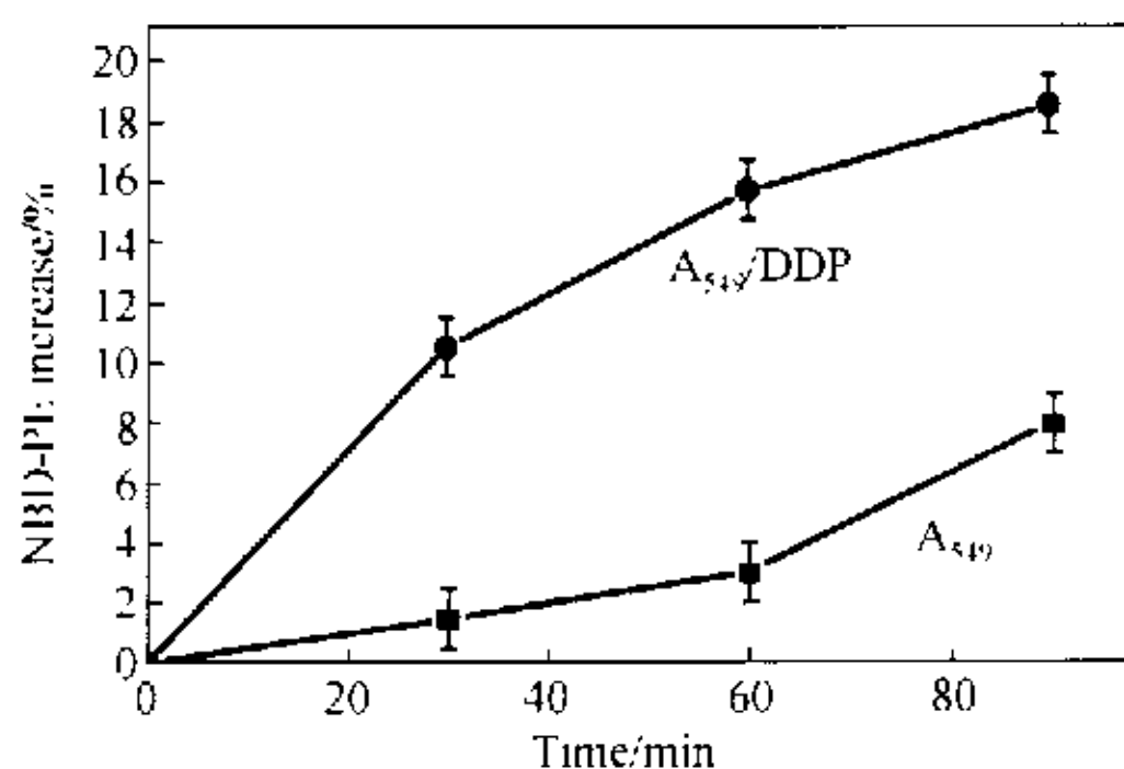
Fig. 2 Phospholipid flippase activity in plasma membrane of sensitive A 549 cells and resistant A 549 /DDP cells.
