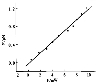
Fig.2 Calibration curve of optical tweezers manipulation force F.
