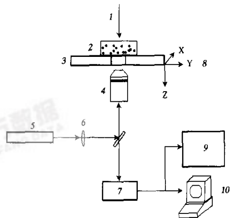
Fig.1 Scheme of the optical tweezers experimental setup 1: illuminate light; 2: sample cell; 3: sample stage; 4: objective; 5: light source of optical tweezers; 6: lens; 7: CCD camera; 8: 3D motion; 9: video recorder; 10: computer.
