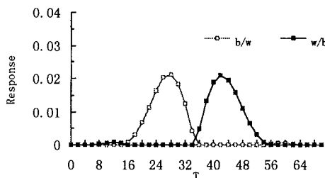
Fig.5. Computer simulation results on "head/tail preference" response of a toad's R3 neuron.
