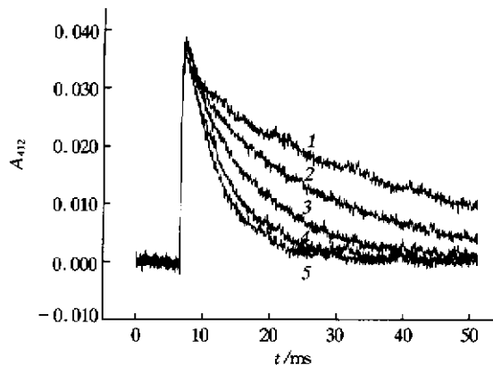
Fig.3 Flash-induced kinetics spectra of the intermediate M_{412} was monitored as the pH shifted from 7.6 to 9.5 1 : pH 9.5 ; 2 : pH 9.1 ; 3 : pH 8.6 ; 4 : pH 8.1 ; 5 : pH 7.6.
