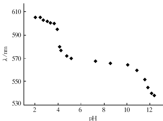
Fig.1 The changes of the wavelength of characteristic absorption peak of bacteriorhodopsin as the pH shifted from 2.1 to 12.3
