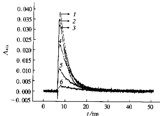
Fig.2 Flash-induced kinetics spectra of the intermediate M_{412} was monitored as the pH shifted from 7.3 to 2.5 1 : pH 7.3 ; 2 : pH 5.9 ; 3 : pH 5.0 ; 4 : pH 3.6 ; 5 : pH 3.0 ; 6 : pH 2.5.
