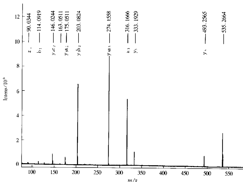
Fig.6 MS/MS spectrum of F-1
