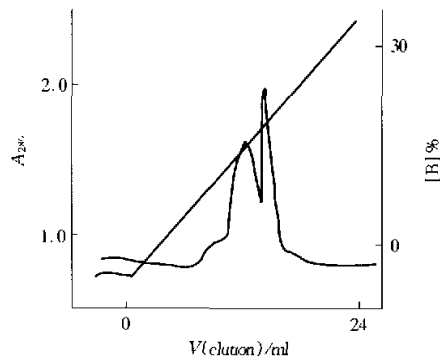
Fig.3 Chromatography of FF on FPLC
