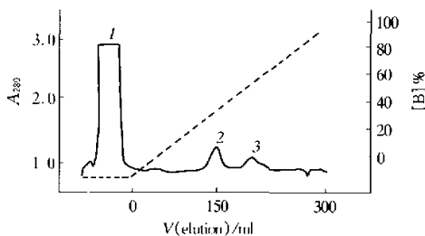
Fig.1 Chromatography of the active fraction with SP-Sepharose Fast Flow 16 /30
