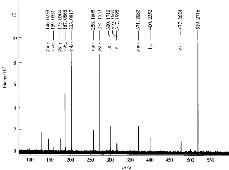
Fig.7 MS/MS spectrum of F-2
