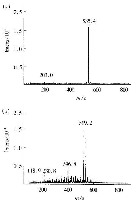
Fig.4 Analysis of F-1 (F-1') and F-2 (F-2') with ESI-MS (a) F-1 (F-1'); (b) F-2 (F-2').
