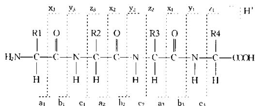
Fig.5 The types of fragment ions observed in MS/MS spectrum The fragment ion which charge is retained on the N terminal is classed as either a, b or c. If on the C terminal, the ion type is either x, y or z. A subscript indicates the number of residues in the fragment.
