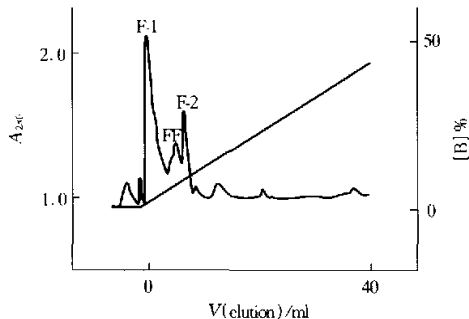
Fig.2 Chromatography of active fraction on FPLC
