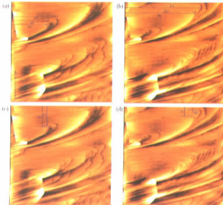
Fig. 1 Series of AFM images taken at 17 min intervals, showing the multi stacked 2D islands and expansion of the stack on the {100} surface of EAFP monoclinic crystal at higher supersaturation
