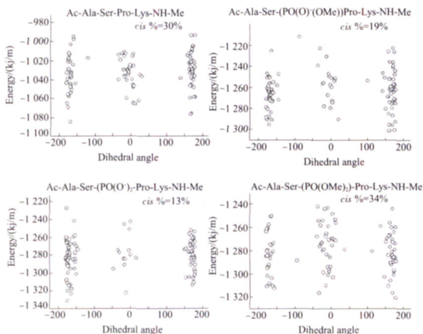
Fig. 7 Low energetic conformation distribution of four tetrapeptides
