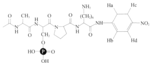
Fig. 2 Protons on benzyl ring tested
