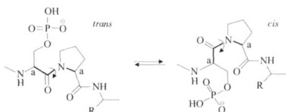
Fig. 1 Peptidyl-prolyl conformation of cis/trans isomers
