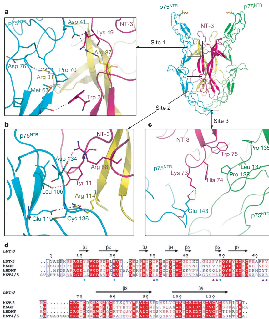
Figure 2 | Interactions between p75 NTR and NT-3. a , Close-up of the site 1 interface. NT-3 monomers are shown in red and yellow, and p75 NTR is shown in blue and green. Hydrogen bonds and salt bridges are shown as dashed lines. b , c , Close-ups of the site 2 ( b ) and site 3 ( c ) interfaces. d , Human (h) neurotrophin family sequence alignments for NT-3, NGF,
