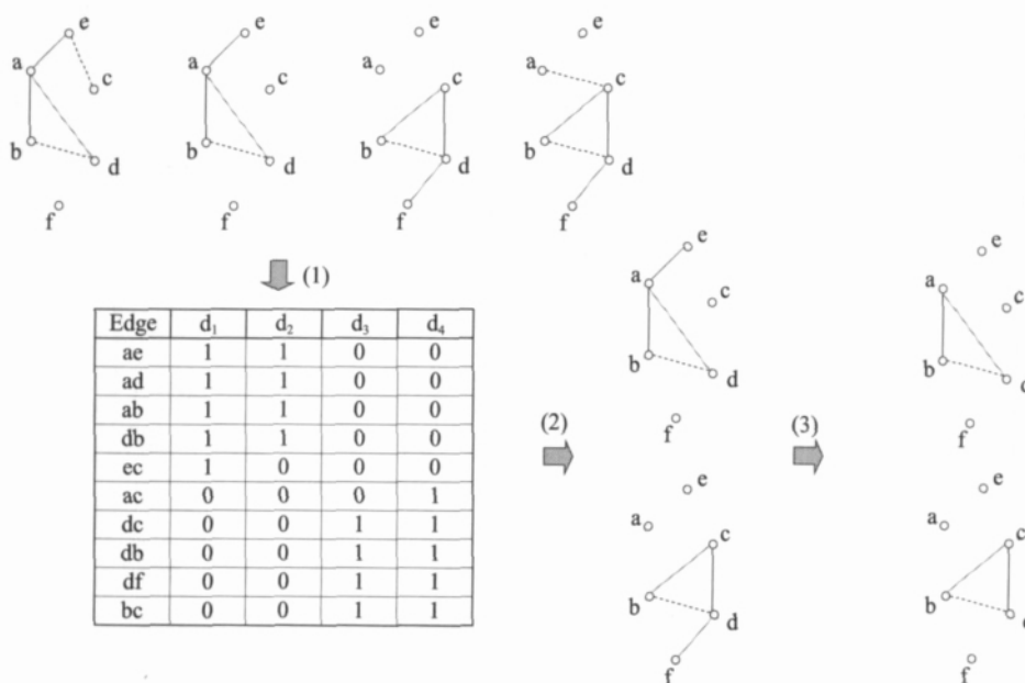
Fig. 2 An example of the “conserved subgraph of multiple networks” method
