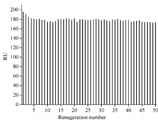
Fig. 2 Surface stability in regeneration cycles. Repeated 5 \mu g ml -1 mAb 8G3 injections (2 min) and surface regeneration using 30 \mu L 20 mM HCl at a flow rate of 10 \mu L min -1 . The stability of the sensor surface was confirmed with a decrease in surface activity of 11.7% after 50 regeneration cycles.
