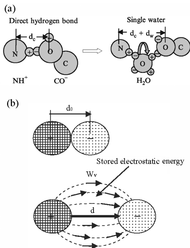
Fig.4. (a) The conceptual diagram showing formation of single water bridges between \text{NH}^+ and \text{CO}^- groups in hydrated proteins and (b) the Work is required to separate a charge pair. The irreducible separation of partial charges on the backbone of macromolecular polymers such as proteins creates an electrostatic field that stores this energy.
