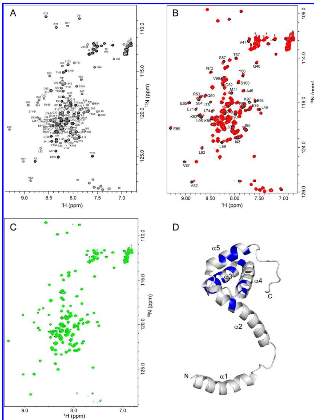
Figure 2. Detecting the binding site of p53(1–96) on PDCD5. (A) 2D ^1\text{H} – ^{15}\text{N} HSQC spectrum of full-length PDCD5 showing the residue-specific assignments of backbone amide groups. The assigned cross-peaks are indicated by labeling the one-letter amino acid code and residue number. (B) 2D ^1\text{H} – ^{15}\text{N} HSQC spectrum of 0.2 mM ^{15}\text{N} -labeled PDCD5 (black) is overlaid with the spectrum recorded for ^{15}\text{N} -labeled PDCD5 mixed with unlabeled p53(1–96) in 1:1 molar ratio (red). (C) Overlay of the 2D HSQC spectra of ^{15}\text{N} -labeled PDCD5 in mixture with unlabeled p53(94–312) (green) and free ^{15}\text{N} -labeled PDCD5 (black). (D) Mapping of the p53(1–96) binding surface on the PDCD5 structure (PDB ID 2K6B). Residues with significant chemical shift differences are shown in blue.
