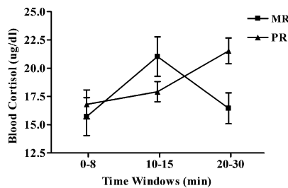
Fig. 3. The time profile of the plasma cortisol response to stress (capture and restraint) for the MR and PR juveniles at 2 y of age. The values are the plasma cortisol levels (mean \pm SEM) measured within the three time windows.
